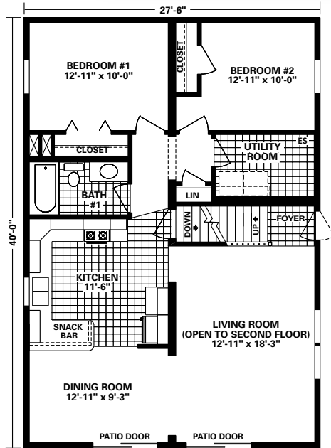
4028-504 40' 1100 Sq. Ft. First Floor
