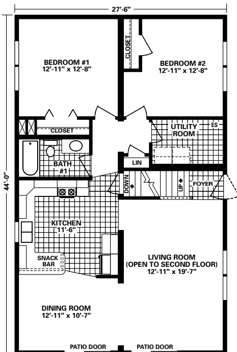
4428-504 44' 1210 Sq. Ft. First Floor
